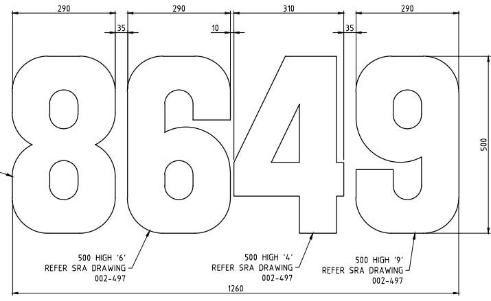
NUMBER SPACING DETAILS SCALE 1:5
